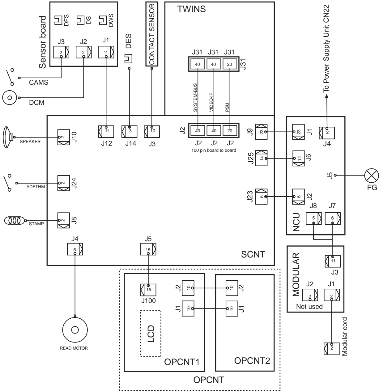
Figure 4-48 Wiring Diagram (1)
