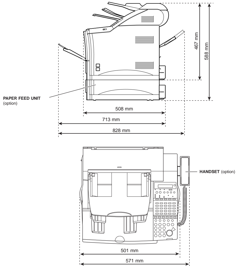
Figure 3-1 External View
