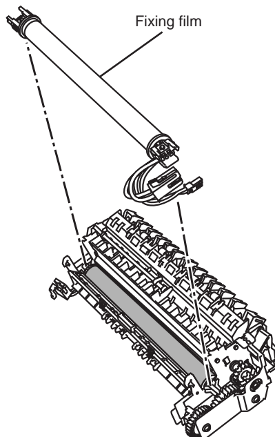
Figure 4-41 Cleaning Location
