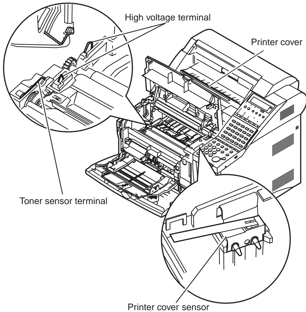
Figure 2-50 Toner Sensor
