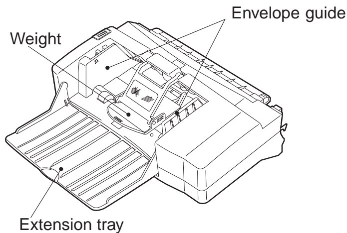
Figure 5-29 External View
