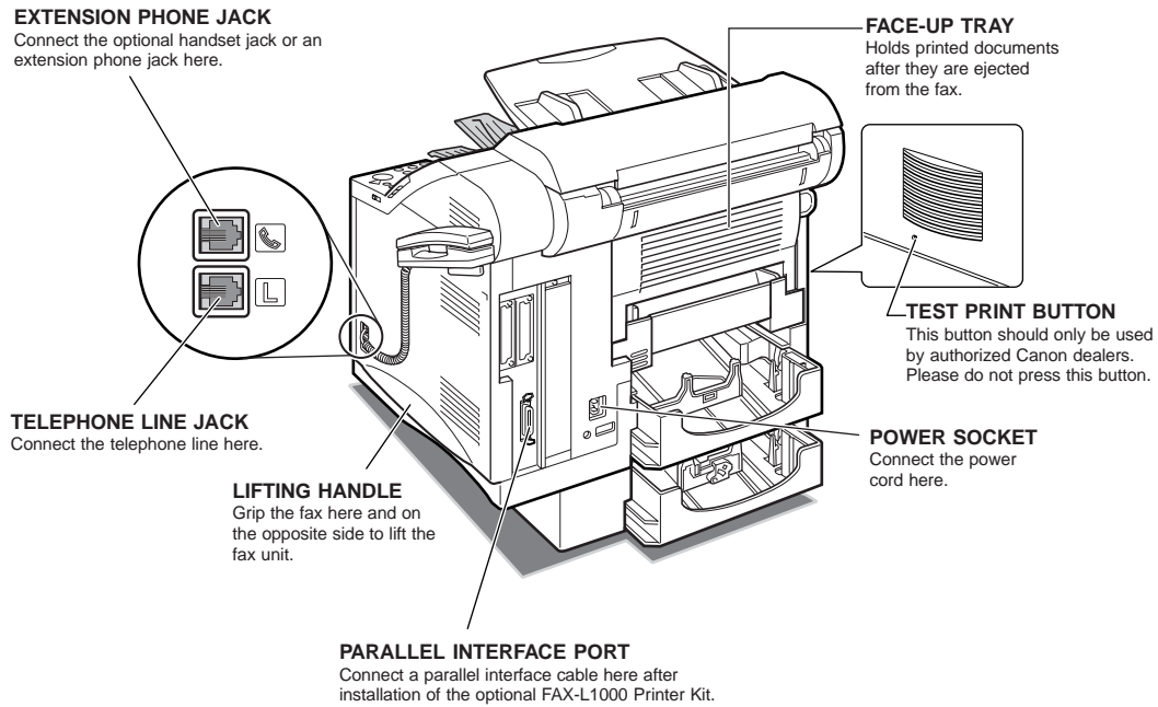
Figure 2-2 Rear View
